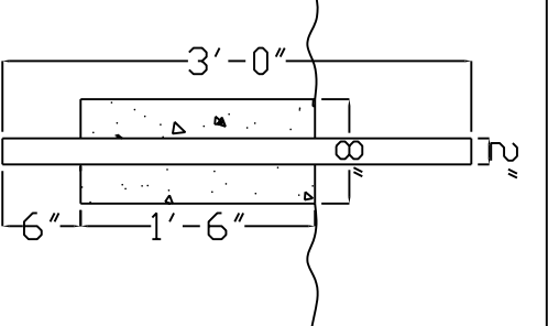
SECTION AT FOOTING
