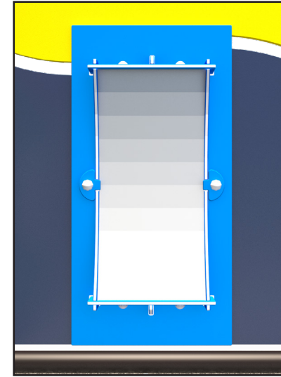
Concave Mirror
