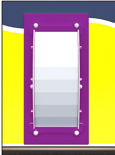
Convex Mirror
