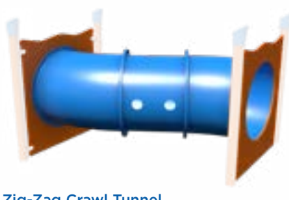
Zig-Zag Crawl Tunnel Left or Right Zig-Zag Ages: 2-5, 5-12 Decks: Equal Height Offset by 24" Available for 5" Posts with 48" Decks or 3.5" Posts with 46.5" Decks
