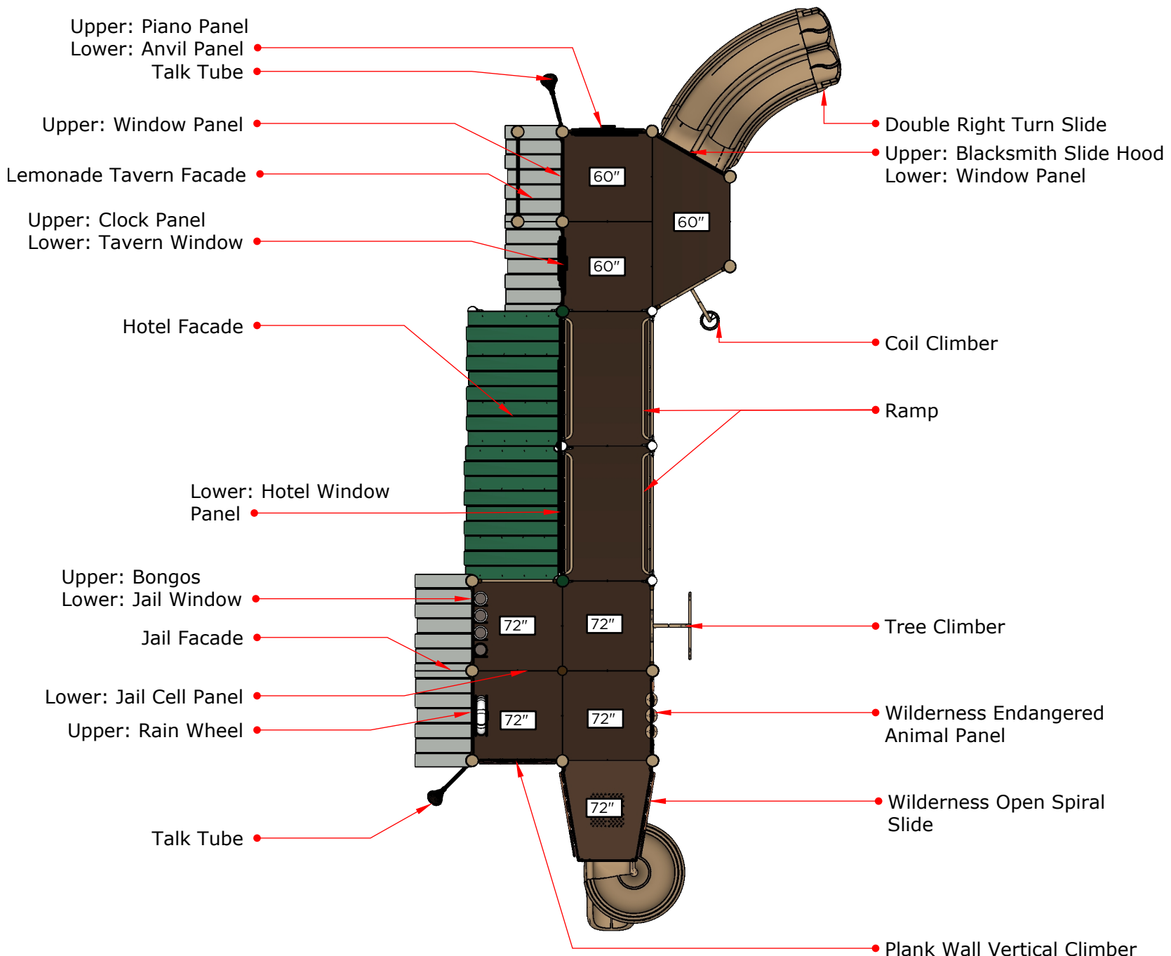
Coastal Village Section 0 5 10 Scale: 1" = 10'
