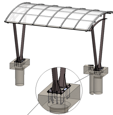
DETAIL OF OPTIONAL FOOTING DESIGN
